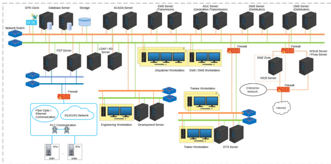
Typical Configuration for Dispatch Control Center
